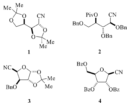
Figure 1. Nitriles 1 – 4 .
